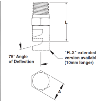
Spray is deflected 75° away from the centerline of the nozzle.
